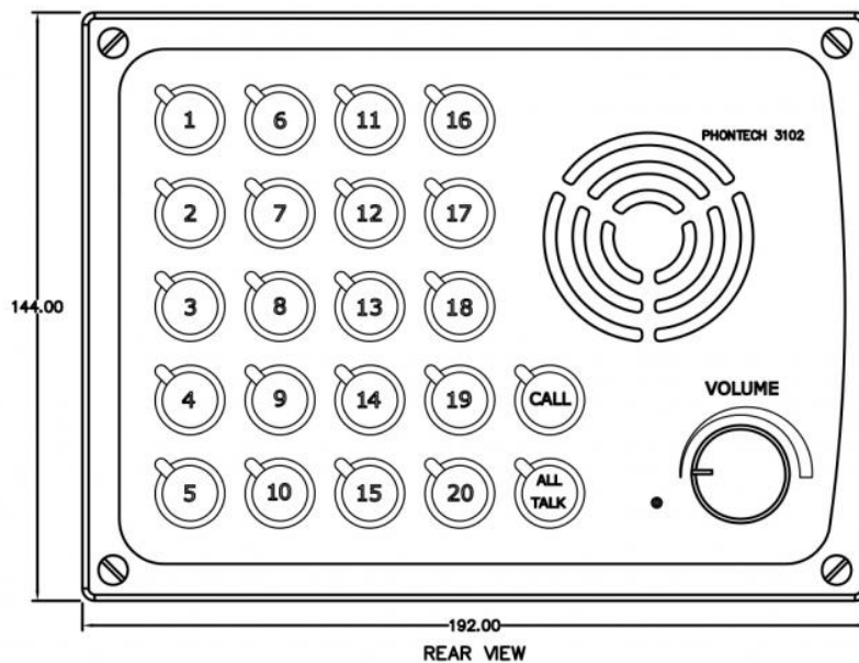
REAR VIEW
