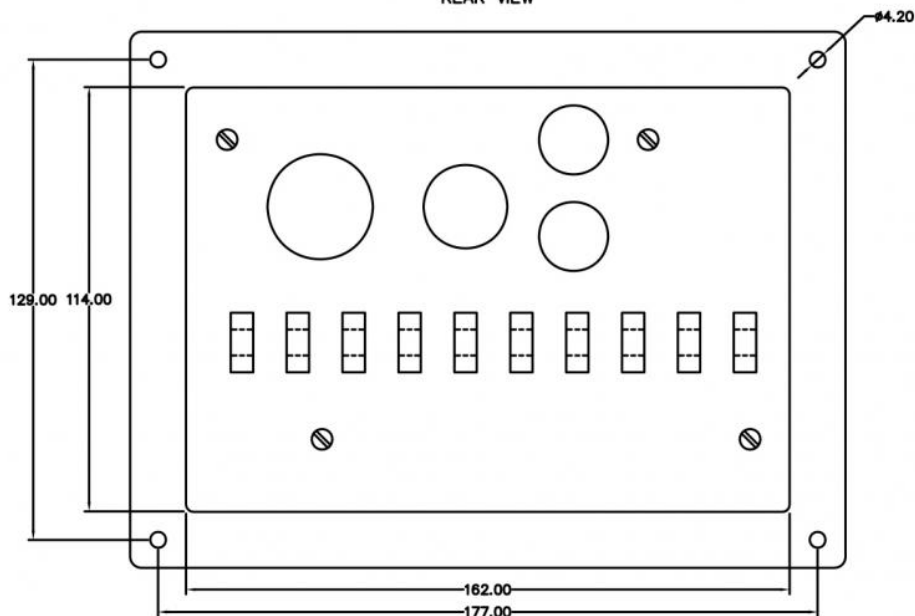
REAR VIEW
